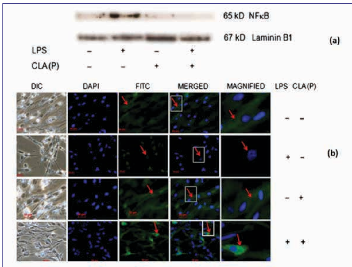
Figure : Effect of CLA pre-treatment on LPS-induced NF-κB activation and immunolocalization: Western blot (a) showed that there was more nuclear NF-κB in nuclear protein isolated from cells treated with LPS, while there was an absence of NF-κB in the protein isolated from cells pre-treated with CLA followed by LPS treatment. Similarly, immuno-staining (b) showed that CLA pretreatment prevented the NF-κB translocation to nucleus, while in LPS treatment (second row from top), there was an intense nuclear NF-κB levels required for pro-inflammatory cytokines expression. Arrows indicate the localization of NF-κB localization in either cytoplasm or nucleus. Boxed regions are magnified further for more clarity. Scale bar, 50 μm. (above figure)
