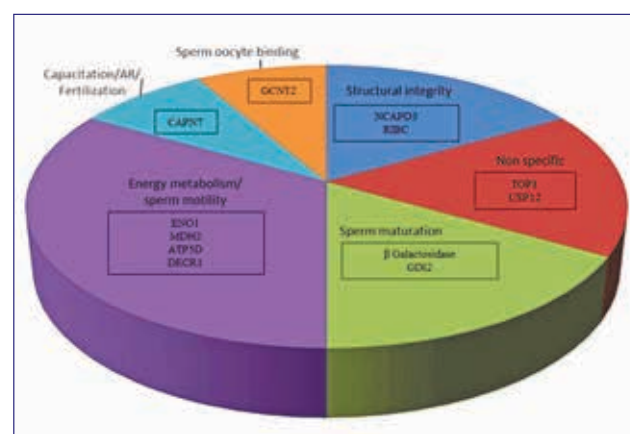
Sperm specific functional classification of proteins under expressed in spermatozoa of low fertile crossbred bulls compared to high fertile bulls
