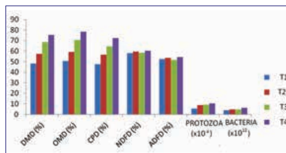
Effect of various levels of MP and ME on digestibility of nutrients and microbial population
