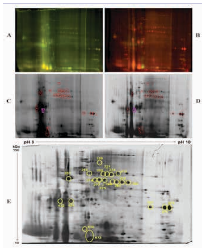
Analysis of sperm proteome by DIGE. [A] Low fertile labeled with Cy3 and high fertile with Cy5. [B] Dye swapped to avoid bias. [C&D] Differentially expressed spots, analysed by DeCyder software. [E] Silver stained preparative gel used for spots identification, differentially expressed protein spots are shown in circles with spot numbers.
