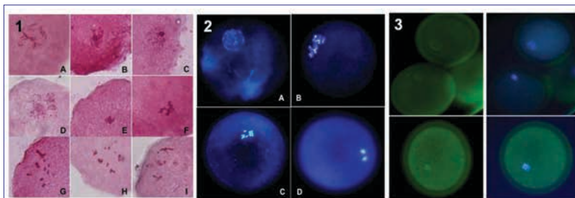
Three alternate methods of characterizing the GVBD event in oocytes. 1. Aseto-orcein staining 2. Hoechst staining and 3. Anti Lamin-DAPI staining. Method 3 was found to be a highly authentic and reproducible one
