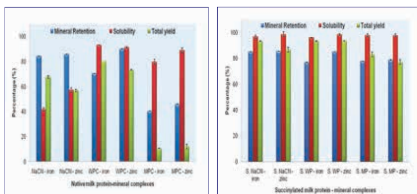
Fig: Mineral retention, solubility and yield (on weight basis) of selected complexes of different mineral bound milk proteins: (a) native protein – mineral complexes (b) succinylated protein – mineral complexes
