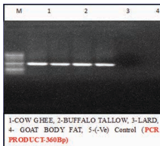
PCR amplification for fat samples using UNI-1 primer
