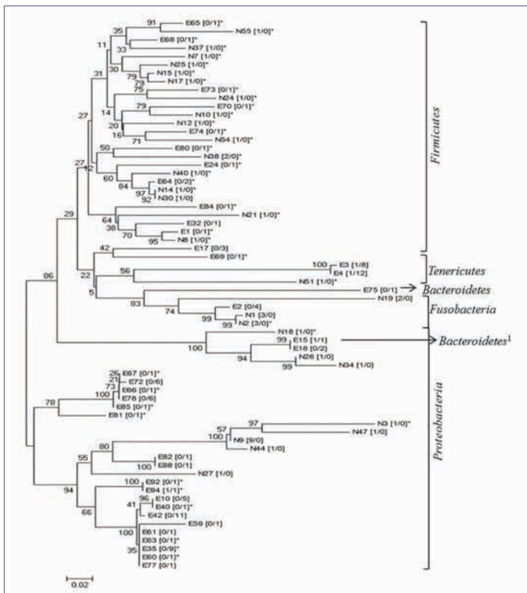
Figure: Phylogenetic tree of the bacterial groups identified from clone libraries from uteri of normal (n=3) and endometritic (n=3) postpartum buffaloes showing their affiliations.
