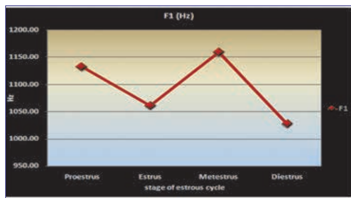
Formants F1 (Hz) trend of voice signals during different stages of estrous cycle in Murrah buffaloes
