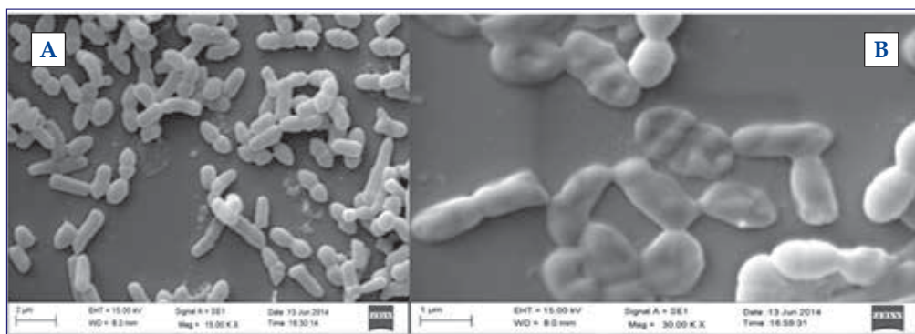
Figure: Scanning electron micrograph of mechanism of action of nanoemulsion on E. coli A) E. coli culture B) E. coli culture treated with emulsion
