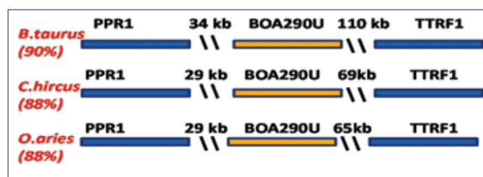
Similarity of the unique long non-coding RNA identified in buffalo oocytes and its location at intergenic region across the species
