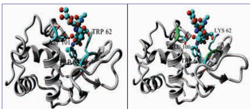
Structural Models of Buffalo SLLP1 with Tri-NAG (left side)
