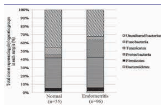
Fig. Stacked bars showing the bacterial group-level compositions of the uteri of normal and endometritic postpartum buffaloes
