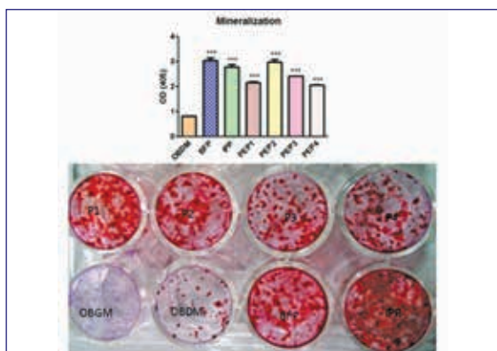
Fig: Plate showing the mineralization nodules of osteoblasts as analyzed by alizarin red staining OBGM: Osteoblast growth medium, OBDM: Osteoblast differentiation medium, BFP: Bone forming peptide, IPP: Isoleucine-Proline-Proline, P1: peptide 1, P2: peptide 2, P3: peptide 3, P4: peptide 4.
