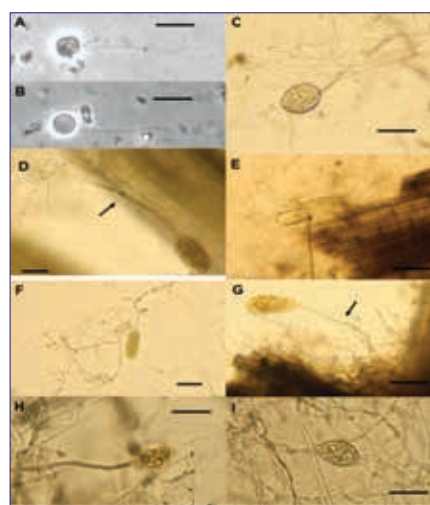
(Figure - Morphology of zoospores of a new anaerobic fungi (A, B) are uniflagellate, with the flagellum ca. 3-4 times the length of the spore body. Thalli are monocentric with sporangia normally being formed terminally (E-I) but occasionally intercalary (D). The shape of the sporangium was variable, ranging from ovoid (C) to elongate (F) and the sporangiophore usually (G-I) 2-3 times the length of the sporangium. A constriction is often visible at the base of the sporangiophore (arrowed, G, I). Scale bar indicates 10 \mu\text{m} (A, B) or 50 \mu\text{m} (C-I).
