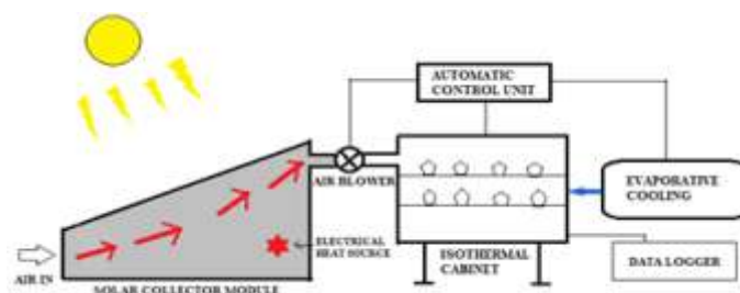
Fig: The conceptual diagram of automatic integrated hybrid solar system for yoghurt
