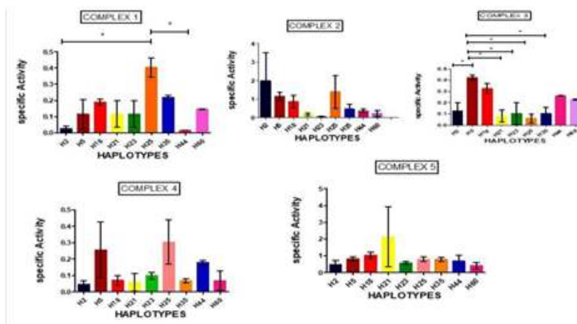
Fig.: Complex I, Complex II, Complex III, Complex IV and Complex V Specific Activity measurements in haplotype-specific different ovarian tissues. The data are presented as the mean \pm SEM. Asterisks indicate the level of statistical significance of differences ( *P < 0.05 ).
