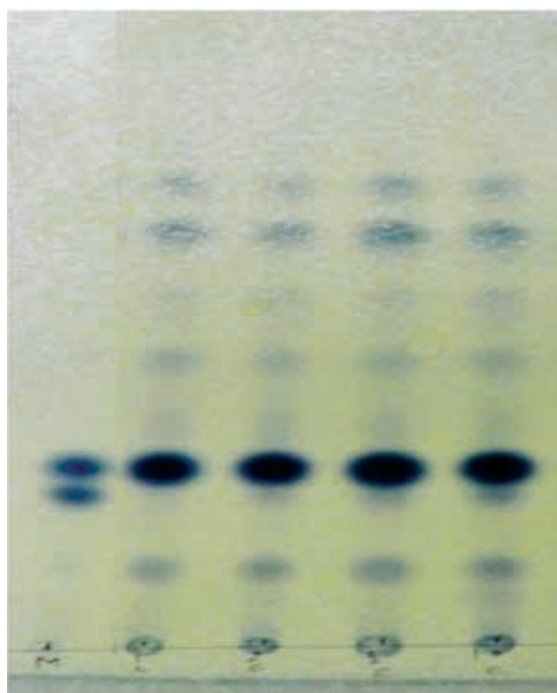
A: cholesterol + \beta -sitosterol; B: Pure ghee; C: 1% groundnut oil in ghee; D: 2% groundnut oil in ghee; E: 5% groundnut oil in ghee
