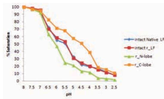
Iron release by recombinant intact Lf, N-lobe and C-lobe of Lf. Curves represent intact native Lf (blue), intact recombinant Lf (red), recombinant N-lobe (green) and C-lobe (orange) of buffalo Lf
