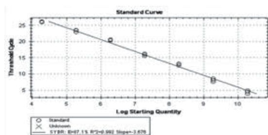
Real Time PCR Graph, Standard Curve and Melt Peaks of R. flavefaciens
